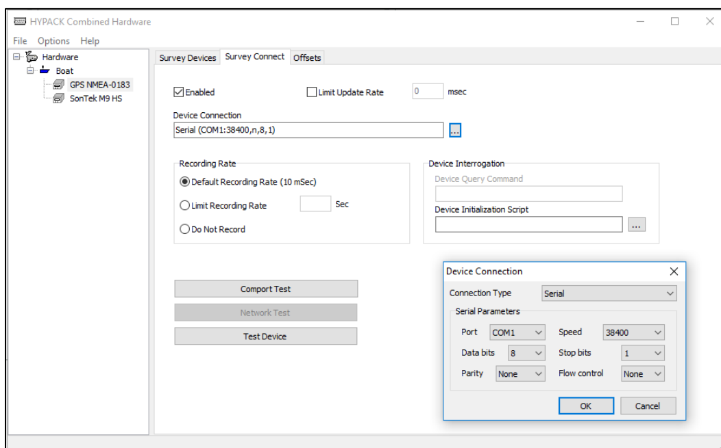
Figure 6.—Survey Connect tab for the selected GPS device within the HYPACK Combined Hardware window.
