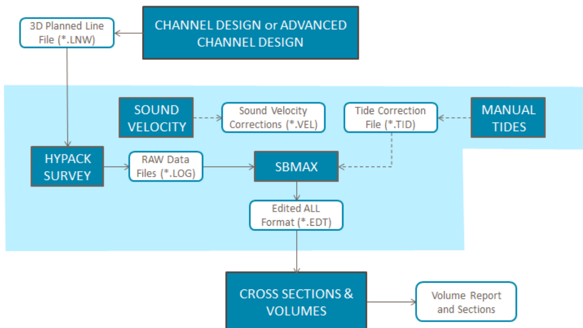
FIGURE 22. Profiles and Volumes in CROSS SECTIONS AND VOLUMES
